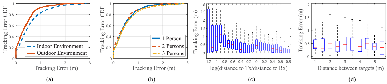
Figure 9: Tracking error analysis over 40 different experiments in 6 different areas (five area pictures shown in this paper and one additional indoor area not shown) and various tracking routes. (a) CDF of tracking errors in outdoor vs indoor environments from tracking 1, 2, and 3 people walking on different tracks, on different days. Performance is better in outdoor environments due to less multipath, as expected. (b) CDF of tracking errors for different number of people. Comparable performance is seen for all cases of 1, 2, or 3 people. (c) Box plot of the distribution of point-wise tracking error over all the experiments as a function of the logarithm of the ratio between the distance of the target to the Tx and its distance to Rx. Targets closer to Rx tend to have lower errors. (d) Box plot of the distribution of point-wise tracking error as a function of the inter-target distance showing little to no effect.
