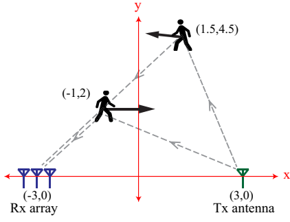
Figure 4: Example of ambiguity resulting from the measurement of \psi = (0.187, 0.707) . Two targets result in the same measurement: one at location (-1,2) with heading of 0^\circ , the other at location (1.5,4.5) with heading of 173^\circ . Both targets have a speed of 1 m/s.
